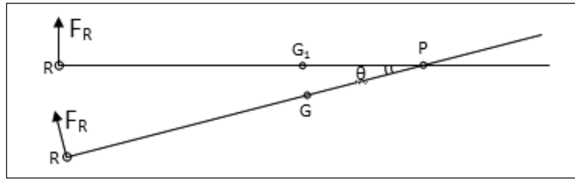
Fig.11 Box Barge Rudder Force applied
