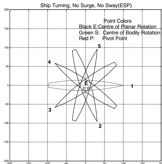
Fig.5 Yaw only
