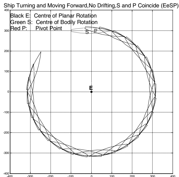
Fig.8 Yaw+Surge
