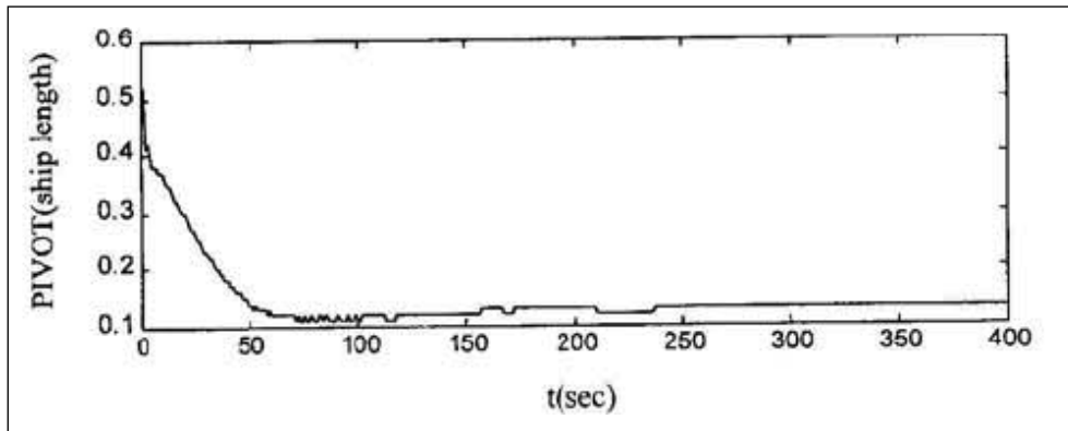
Fig.3 Pivot Point starting from S
