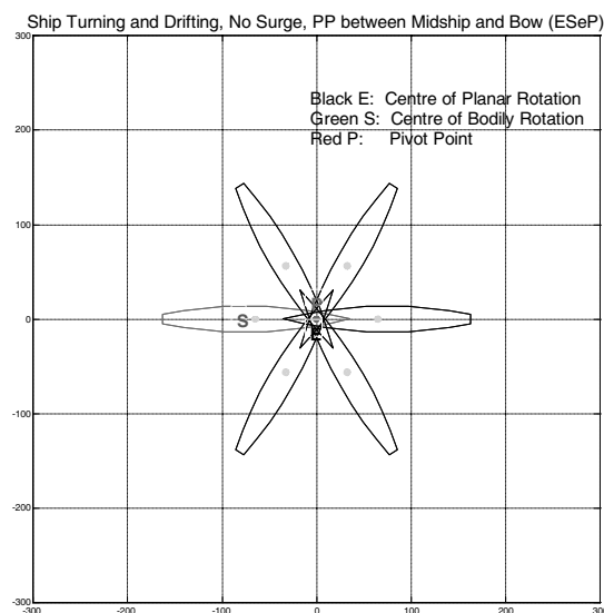
Fig.6 Yaw+Sway
