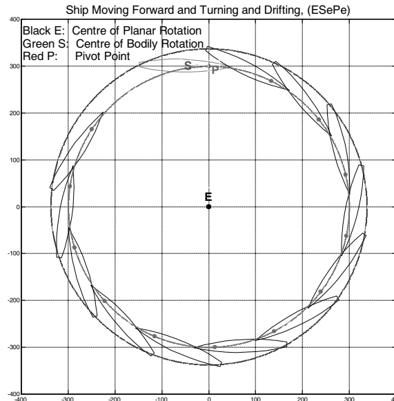
Fig.9 General Planar Motion
