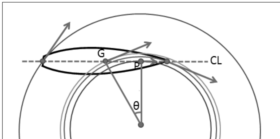
Fig.2 Local Drift Angle, Pivot Point
