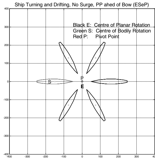
Fig.7 Yaw+Sway
